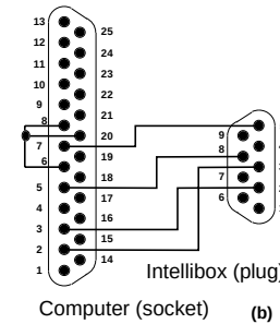
Figure 1.91 Connection of the serial interface
